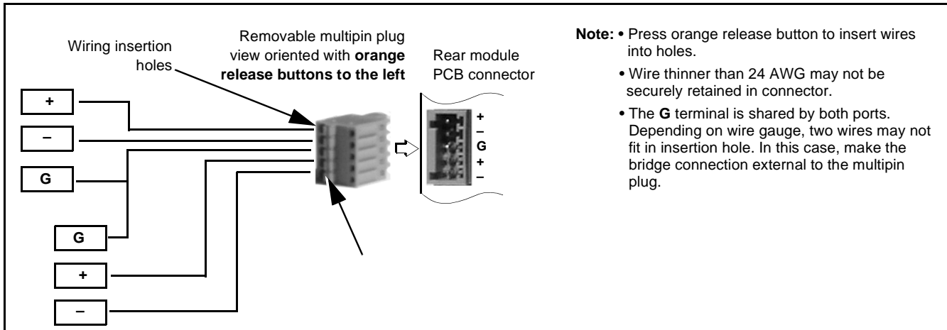
Figure 2-2 Balanced Audio Connector Pinouts
