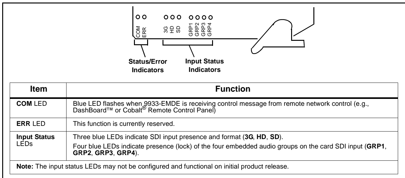
Figure 3-4 9933-EMDE Card Edge Status Indicators
