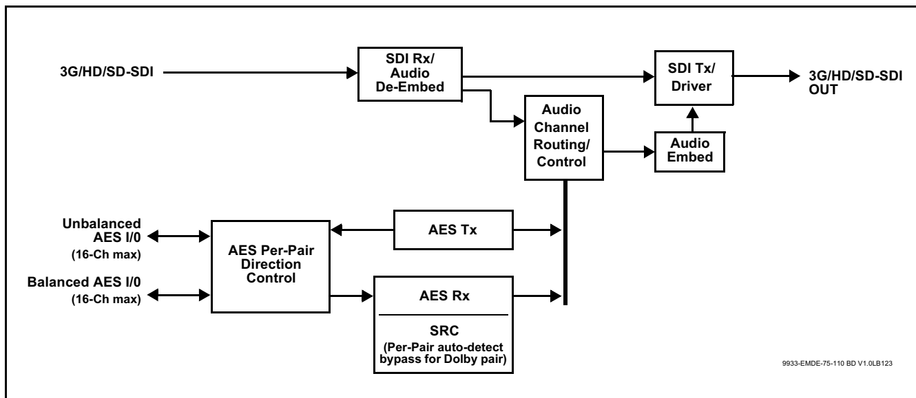
Figure 1-1 9933-EMDE-75/110 Functional Block Diagrams
