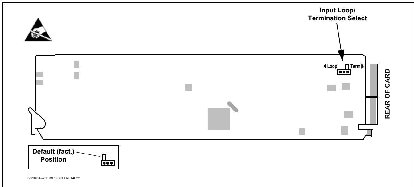
Figure 2-1 9910DA-WC Card Jumpers
