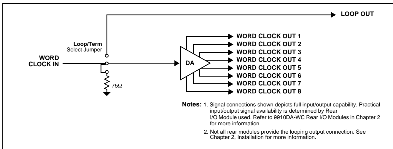
Figure 1-1 9910DA-WC Functional Block Diagram
