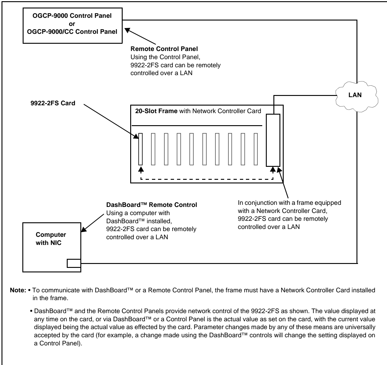
Figure 1-5 9922-2FS User Control Interface
