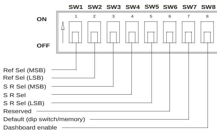
Figure 4. DIP Switch
