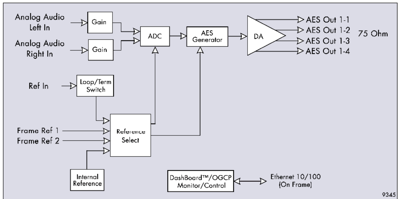
Figure 1. Simplified Block Diagram of the 9345 Functions
