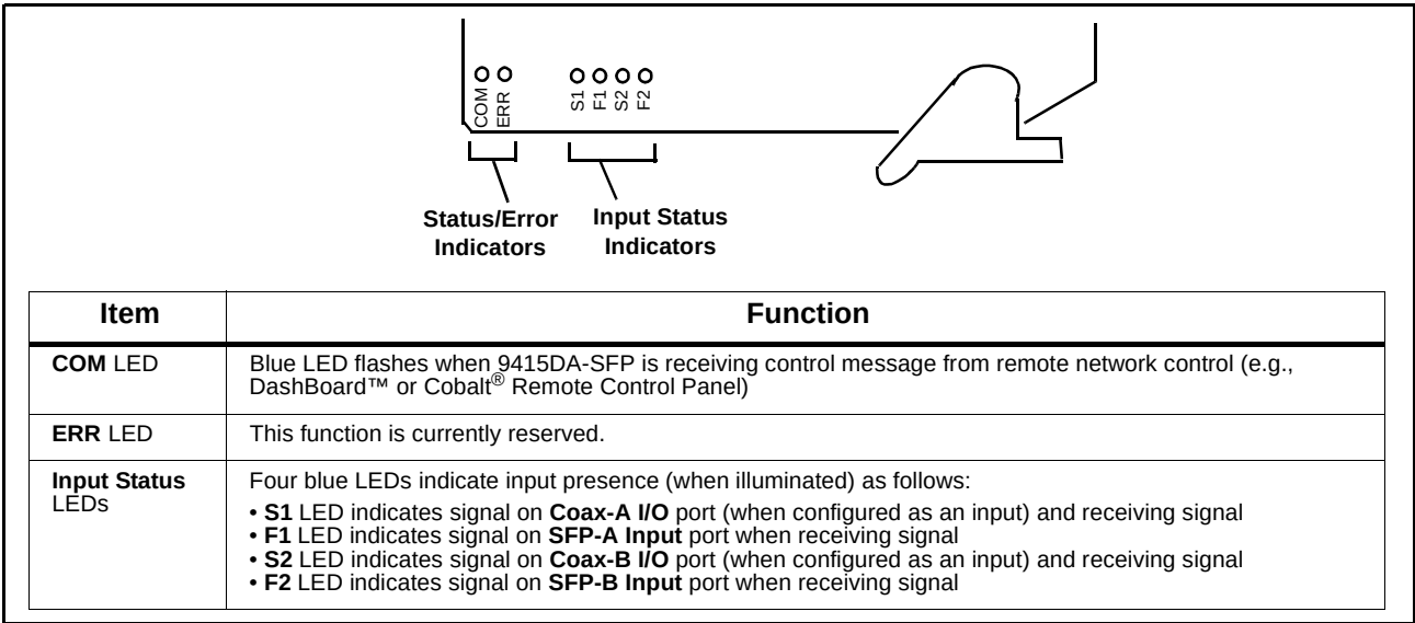
Figure 3-4 9415DA-SFP Card Edge Status Indicators
