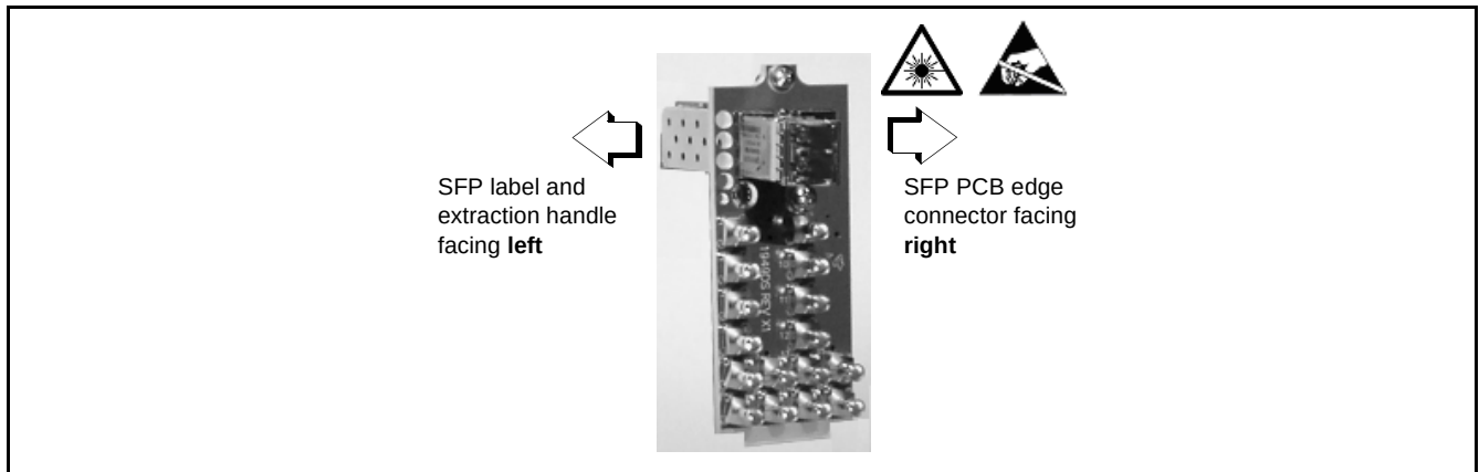
Figure 2-2 SFP Installation Into Rear Module SFP Cage
