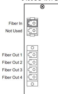
9490OS-1X4-LC
