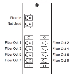
9490OS-1X8-LC
